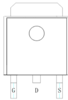
Pin Assignment
